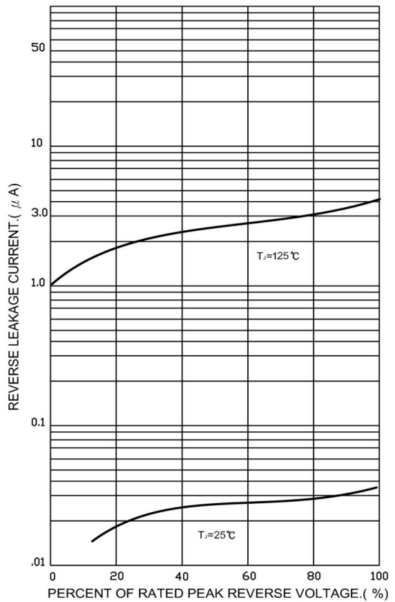
FIG.4-TYPICAL REVERSE CHARACTERISTICS
